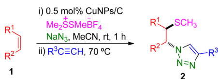
Scheme 2. Optimized Conditions for the One-Pot Synthesis of Triazoles from Alkenes Catalyzed by CuNPs/C
